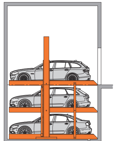
System lowered
