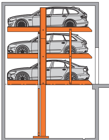
System lifted
